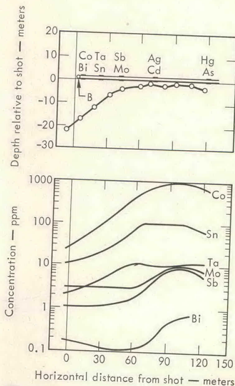
Fig. 7. The chemical tracers and their distribution. Upper figure: Location of chemical tracers in the tunnel and location of postshot samples. Lower figure: Analysis of the final tracer distribution.
