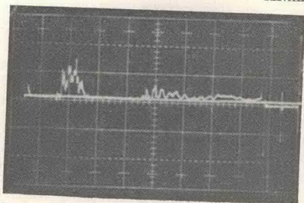
Fig. 5. Cavity gas-pressure instrumentation gage signal from alcove 4: 100-kpsi-range Norwood gage, 2 msec/cm, 25 kpsi/cm.
