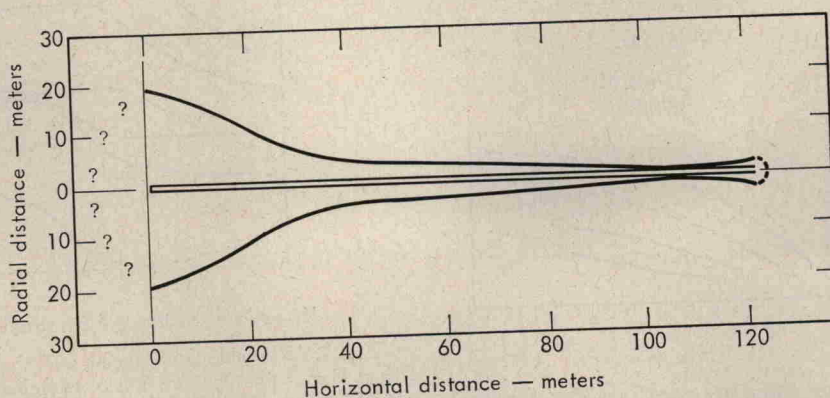
Fig. 8. Shape of the cavity before collapse, inferred from the postshot drilling data.
