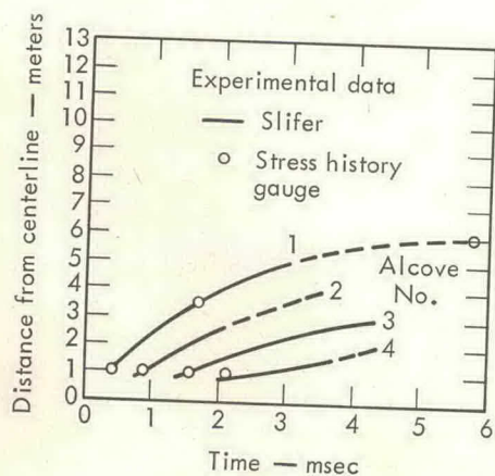
Fig. 6. Slifer and stress gage TOA data for shock-front position in the alcoves.
